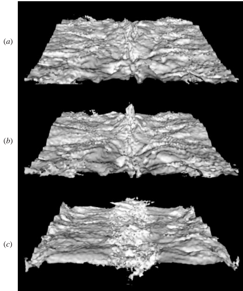
FIGURE 13. Visualization of the isosurface corresponding to one of the nodal planes of the forcing ( g^*(\rho - \rho_0)/\rho_0 = \pi/2 ) for a sequence of times during the formation of spouts. View taken along the x -axis. The time sequence is (a) 15.90T_F , (b) 16.04T_F and (c) 16.32T_F .
