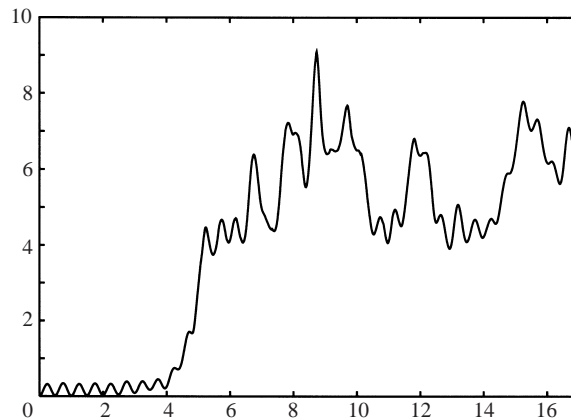
FIGURE 5. Graph of the evolution of the total enstrophy in units of N^2 . The unit for the horizontal time axis is the period of the cyclic forcing, that is \sqrt{2}(2\pi/N) .
