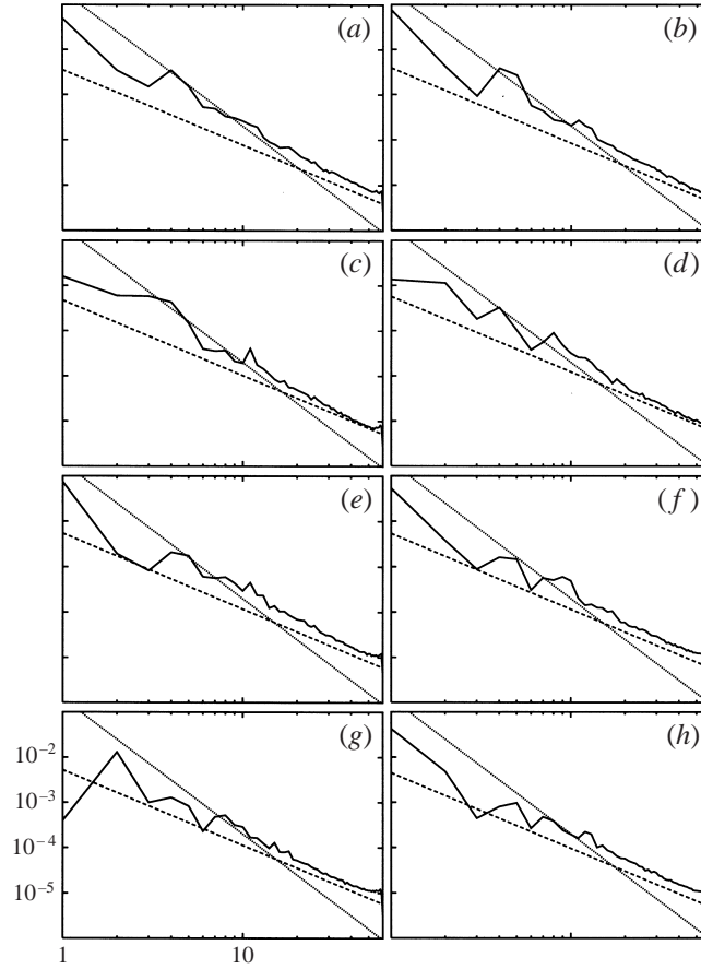
FIGURE 8. Potential energy spectra one cycle of the forcing. In each panel, the dashed line is the Corrsin–Obukhov spectrum C_o \epsilon_{pe} \epsilon^{-1/3} k^{-5/3} with C_o = 0.67 and the dotted line is the saturation spectrum 0.2N^2 k^{-3} . The time interval between frames is \Delta T_F/7 and (a) corresponds to time t = 11.39T_F . These are log-log plots of PE(k) in units of N^2(L/2\pi)^3 vs. k in units of 2\pi/L . All plots have the scales as indicated in panel (g).
