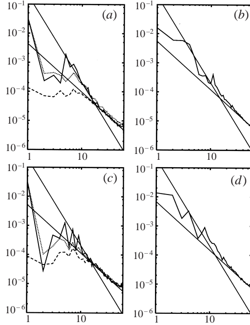
FIGURE 9. (a) Kinetic energy spectra for all three components of the velocity at time t = 11.68T_F . The thick dashed, solid and dotted lines correspond to the energy spectra for the u, v , and w components respectively. The thin solid lines correspond to the Kolmogorov spectrum (1/3)C_K \epsilon^{2/3} k^{-5/3} with C_K = 1.4 and the saturation spectrum 0.2N^2 k^{-3} . (b) Potential energy spectrum at time t = 11.68T_F . The thick solid line corresponds to the potential energy spectrum. The thin solid lines correspond to the Corrsin–Obukhov spectrum C_o \epsilon_{pe} \epsilon^{-1/3} k^{-5/3} with C_o = 0.83 and the saturation spectrum 0.2N^2 k^{-3} . (c) As in (a) but for t = 11.82T_F and C_K = 1.4 . (d) As in (b) but for t = 11.82T_F and C_o = 0.80 .
