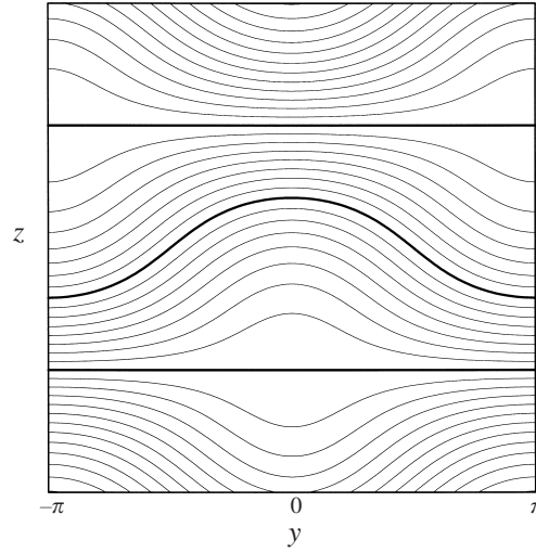
FIGURE 4. Contour plot of the density field in a vertical y, z cross-section through the centre of the domain. The width and height of the cross-section are each 20 m. The instant shown corresponds to maximum displacement of the isopycnals for the forcing of strength S_{GM}(20\text{ m}) as discussed in §3. The upper and lower flat thick contour lines are the isopycnals corresponding to the two nodal planes of the forcing. The curved thick line is the isopycnal that is most strongly disturbed by the forcing and corresponds to \rho = \rho_0 . The contour interval is \pi N^2/16g .
