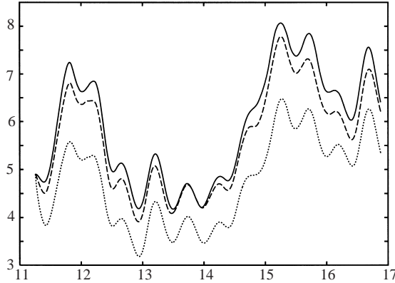
FIGURE 17. Graph of the evolution of the total enstrophy for three different parameterizations of the dissipation: the solid curve corresponds to the case with a_1 = 0.15 , a_2 = 5 , and v_{mol} = 0 ; the long-dashed curve corresponds to the case with a_1 = 0.15 , a_2 = 5 and v_{mol} = 0.01 \text{ cm}^2 \text{ s}^{-1} ; and the short-dashed corresponds to the case with a_1 = 0.267 , a_2 = 9.21 and v_{mol} = 0 . The enstrophy is given in units of N^{-2} , and the unit for the horizontal time axis is the period of the cyclic forcing, that is \sqrt{2}(2\pi/N) .
