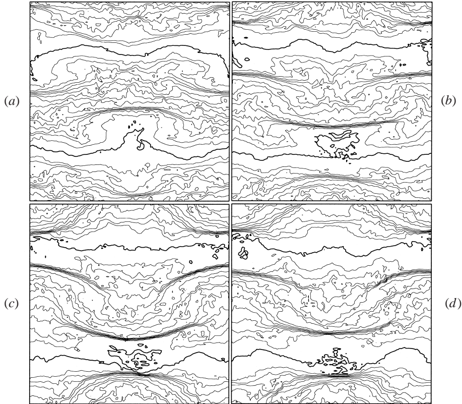
FIGURE 15. Contour plots of density in a vertical y, z cross-section through the domain during half of a forcing cycle to illustrate action of vertical compressional strain on the lower nodal surface. As in figure 14 except for the sequence of times: (a) 16.18T_F , (b) 16.32T_F , (c) 16.46T_F and (d) 16.60T_F .
