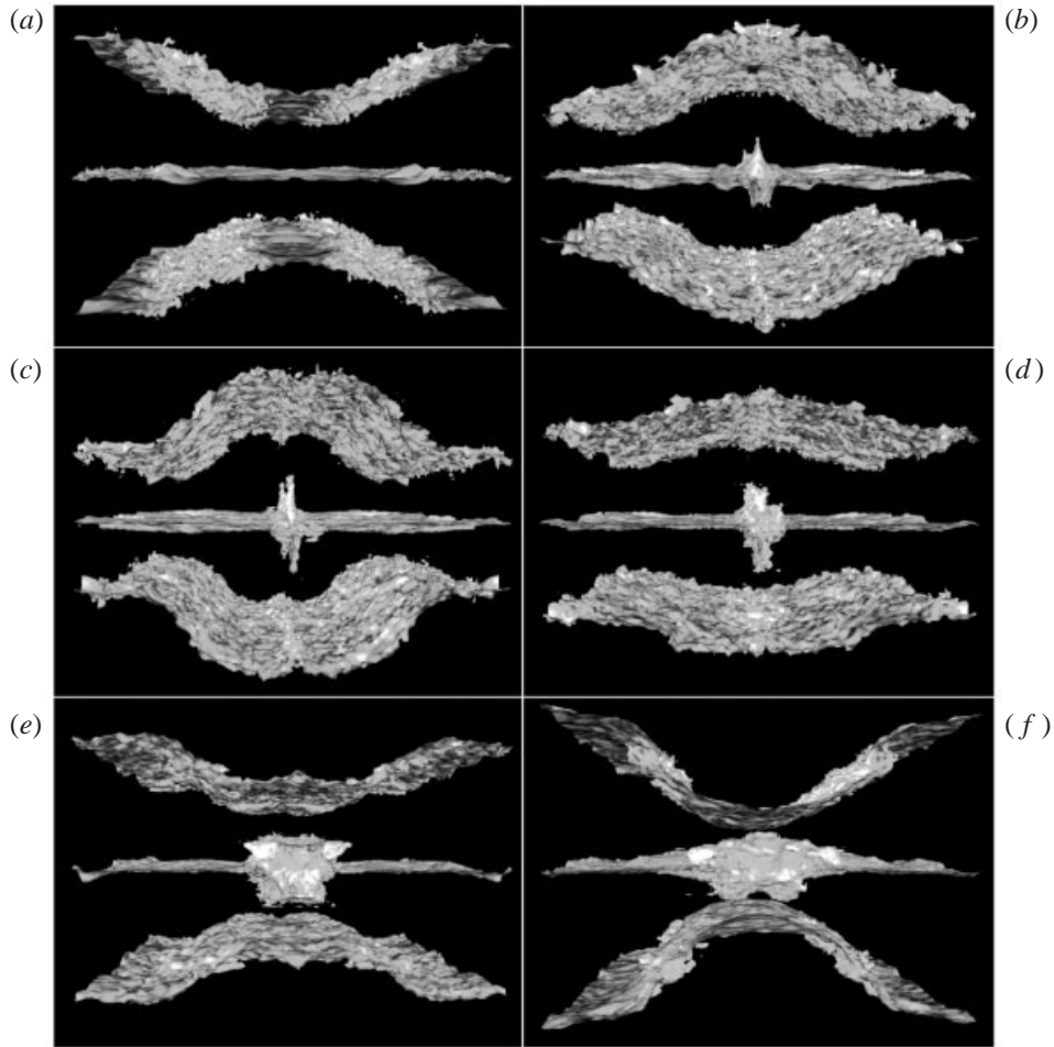
FIGURE 12. The evolution of three density isosurfaces ( g^*(\rho - \rho_0)/\rho_0 = 0, \pi/2, \pi ) showing the evolution of ‘spouts’ from a ‘nodal surface’ and their subsequent collapse with considerable broadening and mixing. Times represented are t = 12.1T_F, 12.4T_F, 12.5T_F, 12.7T_F, 12.8T_F, and 13.1T_F .
