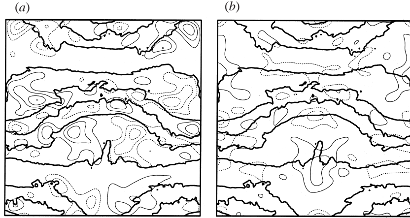
FIGURE 16. Contour plots of the density \rho/\rho_0 (thick lines) in a y, z cross-section at time t = 16.04T_F , as in figure 14 d , with superimposed vorticity and strain fields from t = 15.9T_F (see text). (a) Contour plot of \omega_x , filtered at the 2 m scale, superimposed on the contours of density. The thin solid/dashed lines represent positive/negative contour levels (contour interval 1.1S_G (20 m)). (b) Contour plot of \partial w/\partial z , filtered at the 2 m scale, superimposed on the contours of density (contour interval 0.65S_G (20 m)).
