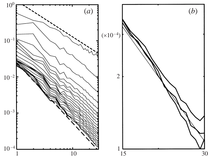
FIGURE 3. (a) Graphs of the potential energy spectra during a decay experiment ( 64^3 ). The thick dashed straight lines indicate k^{-5/3} and k^{-1} spectra. (b) The potential energy spectrum for three decay experiments differing only in the turbulent Prandtl number. The lower/middle/upper spectrum corresponds to the choice Pr_t = 0.50, 0.55, 0.60 . The thin straight line indicates a k^{-5/3} spectrum. The x-range is k = 15 to k = 30 .
