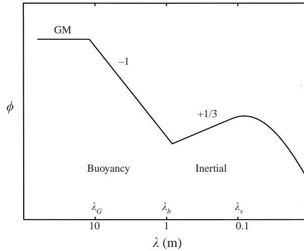
FIGURE 1. Schematic of the oceanic horizontal shear spectrum. The horizontal axis is labelled in terms of wavelength for convenience, but it is actually the k_z wavenumber axis. The slopes corresponding to the k_z^{-1} buoyancy range and the k_z^{1/3} inertial range are labelled by the exponents.
