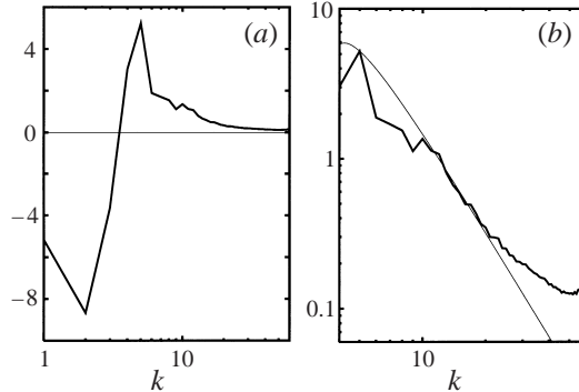
FIGURE 11. (a) The buoyancy flux spectrum averaged over 6 periods of the forcing, with 10 samples per period. (b) As in (a) but only the positive portion of the spectrum plotted in log-log format to compare with the theoretical spectrum of equation (3.8) with negative coefficient D . The result from the simulation is represented by the thick line, while the theoretical spectrum, based on \epsilon_0 = \bar{\epsilon} where the overbar represents time averaging, is drawn as a thin line. All graphs in (a) and (b) are normalized by \bar{\epsilon}/\kappa_b .
