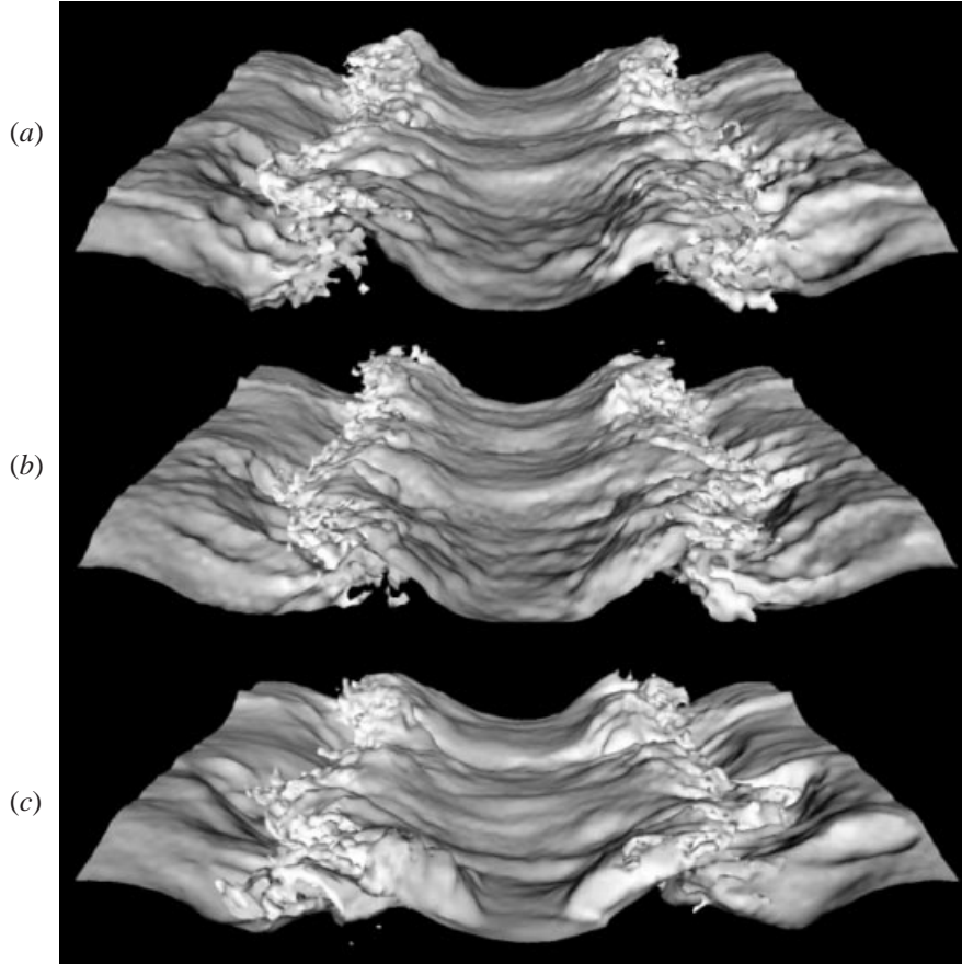
FIGURE 18. A breaking event visualized on the \rho = \rho_0 isopycnal at time 15.3T_F . The three surfaces shown are the same isopycnal level at the same time but for the three different dissipation parameterizations discussed in the text. (a) a_1 = 0.15 , a_2 = 5 , \nu_{mol} = 0 , \kappa_{mol} = 0 . (b) a_1 = 0.15 , a_2 = 5 , \nu_{mol} = 0.01 \text{ cm}^2 \text{ s}^{-1} , Pr_{mol} = 7 . (c) a_1 = 0.267 , a_2 = 9.21 , \nu_{mol} = 0 , \kappa_{mol} = 0 .
