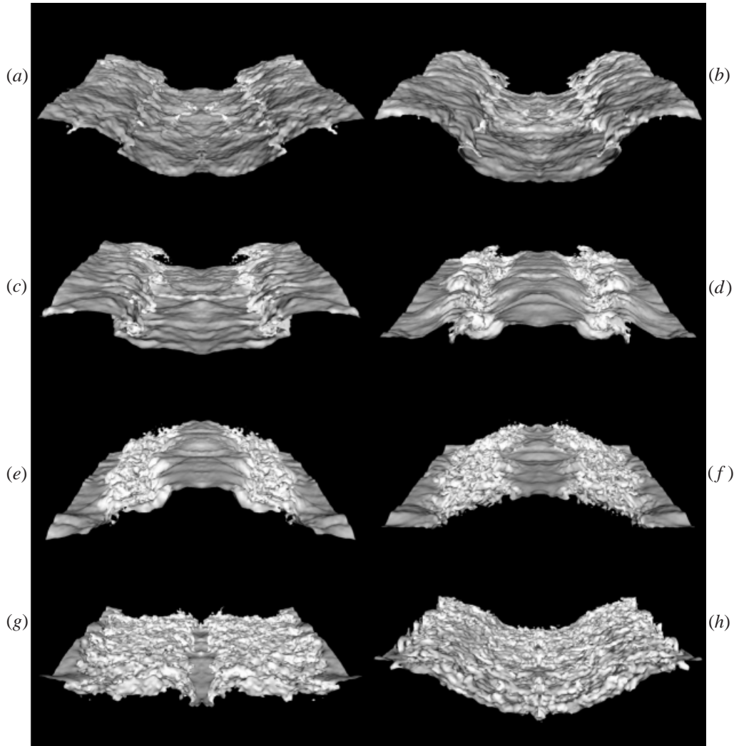
FIGURE 6. The evolution of the \rho = \rho_0 isopycnal during one cycle of the forcing. The frames are ordered by time from (a) to (h). The first corresponds to t = 11.39T_F , the interval between frames is \Delta t = T_F/7 .
