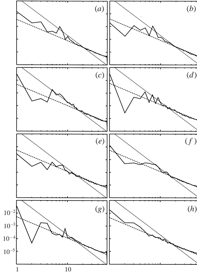
FIGURE 7. Kinetic energy spectra for the v -component of the velocity during one cycle of the forcing. In each panel the dashed line is the Kolmogorov spectrum (1/3)C_K\epsilon^{2/3}k^{-5/3} with C_K = 1.5 , and the dotted line is the saturation spectrum 0.2N^2k^{-3} . The time interval between frames is \Delta T_F/7 and (a) corresponds to time t = 11.39T_F . These are log-log plots of E(k) in units of N^2(L/2\pi)^3 vs. k in units of 2\pi/L . All plots have the scales as indicated in panel (g).
