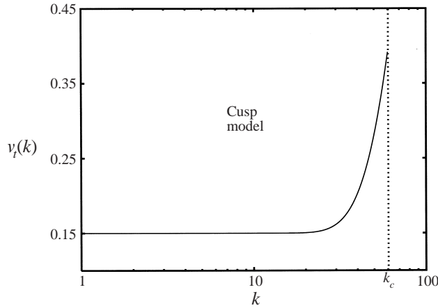
FIGURE 2. Graph of the eddy viscosity divided by (E(k_c)/k_c)^{1/2} , where k_c is the numerical cutoff or truncation wavenumber.
