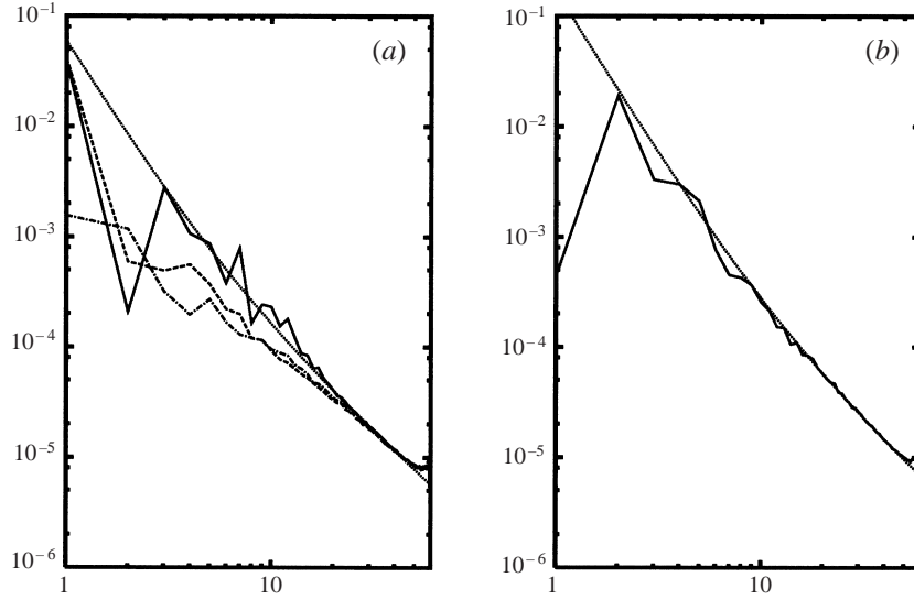
FIGURE 10. (a) Kinetic energy spectra for all three components of the velocity at time 16.8T_F just after a wave breaking event. The dot-dashed, solid and dashed lines correspond to the energy spectra for the u , v , and w components respectively. The dotted straight line corresponds to 1/3 of the theoretical spectrum in (3.5) with C_K = 1.44 and C_u = 0.16 . (b) Potential energy spectrum at time 16.8T_F . The solid line corresponds to the potential energy spectrum. The dotted straight line corresponds to the theoretical spectrum in (3.6) with C_o = 0.73 and C_\theta = 0.16 .
