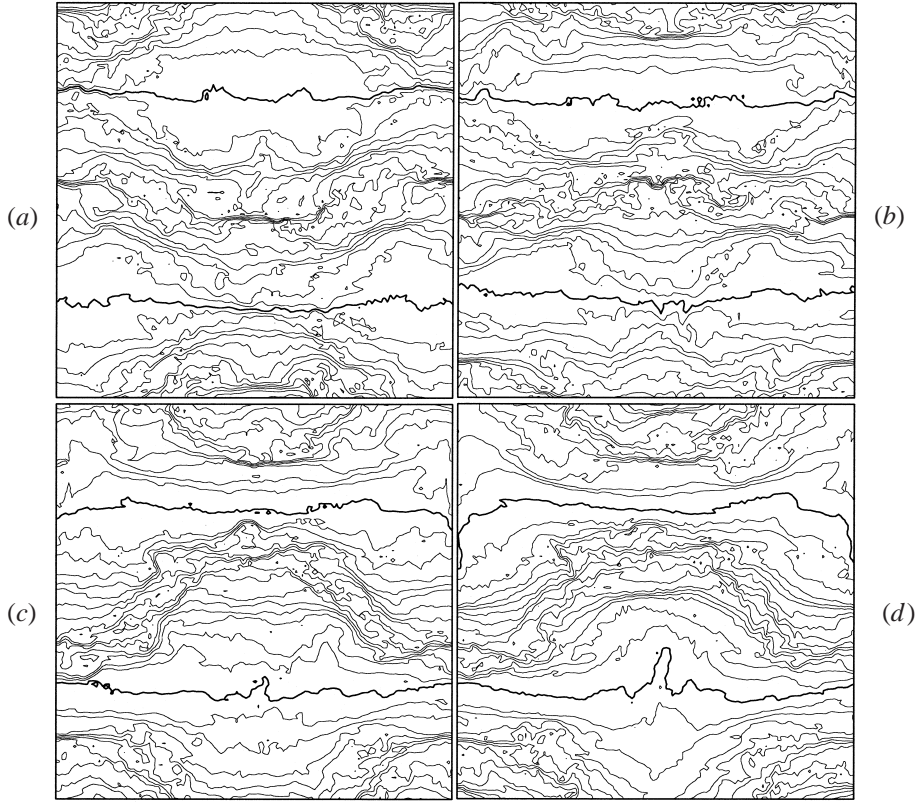
FIGURE 14. Contour plots of density in a vertical y, z cross-section through the domain during half of a forcing cycle to illustrate action of vertical dilational strain on the lower nodal surface. The origin is taken as the centre of each panel. The y - and z -axes are horizontal and vertical respectively. The thick contour lines correspond to isopycnals with the same densities as the nodal surfaces of the forced standing wave. In non-dimensional units these are g^*(\rho - \rho_0)/\rho_0 = \pm\pi/2 . The sequence of times represented is (a) 15.61T_F , (b) 15.76T_F , (c) 15.90T_F and (d) 16.04T_F .
