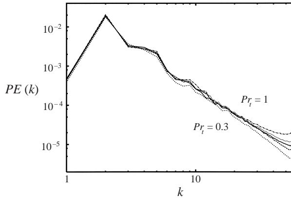
FIGURE 20. The potential energy spectrum at time 16.8T_F for each of five runs representing different choices of Pr_t . For all cases v_{mol} = 0.01 \text{ cm}^2 \text{ s}^{-1} and Pr_{mol} = 7 . The values of Pr_t are 0.3 (short-dash), 0.4 (long-dash), 0.55 (solid), 0.6 (dots), and 1.0 (dot-dash). The correspondence of these values with the graphs is such that the lower the value of Pr_t , the lower the value of the energy at the upper wavenumber cutoff.
